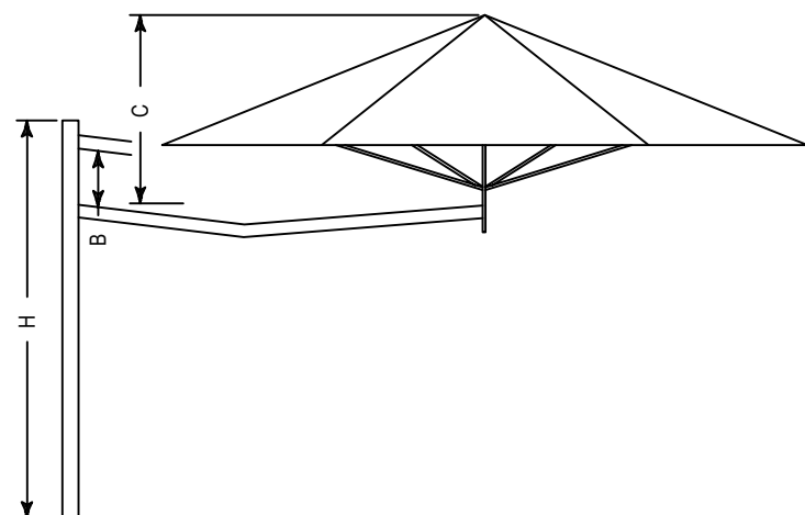
FRONT VIEW - HIGH
