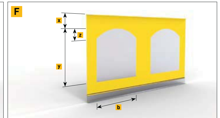
Side sheet with one arched window per segment
